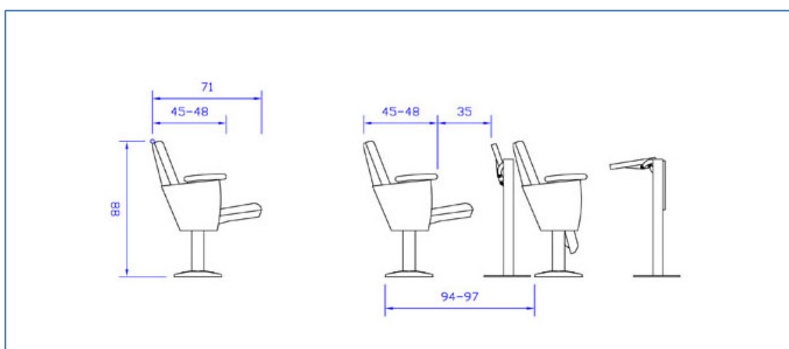
Light with individua Anti-Panic table
