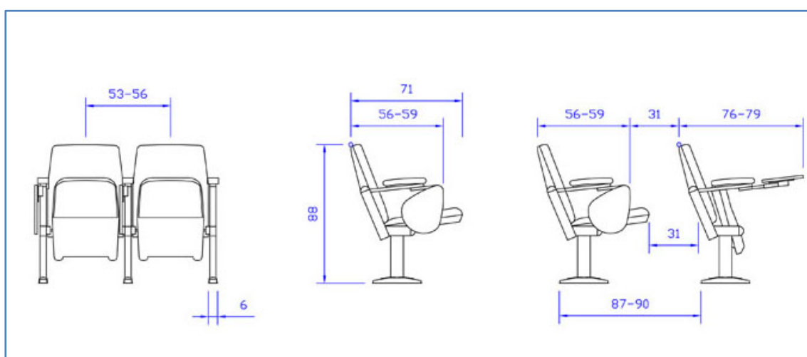
Light with Anti-Panic writing tablet
