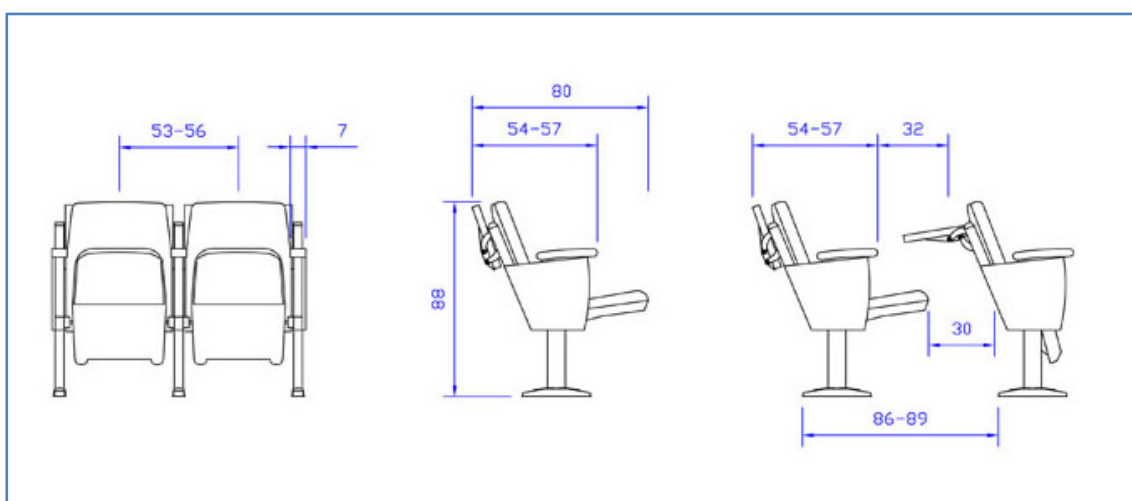
Light with Anti-Panic table
